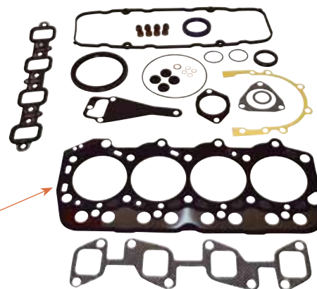
Kit joints complet - Overhaul Gasket Kit 041112032171 J5398K
